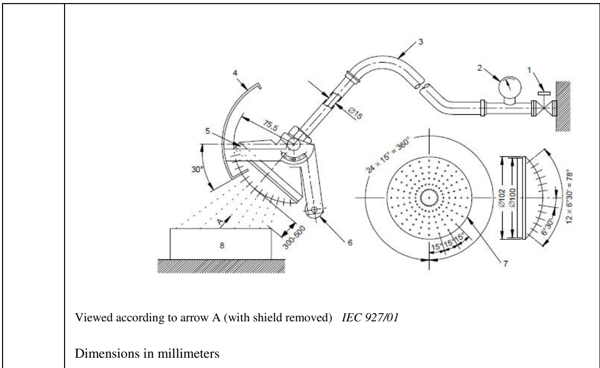
Figure 2 Splashing test nozzle
