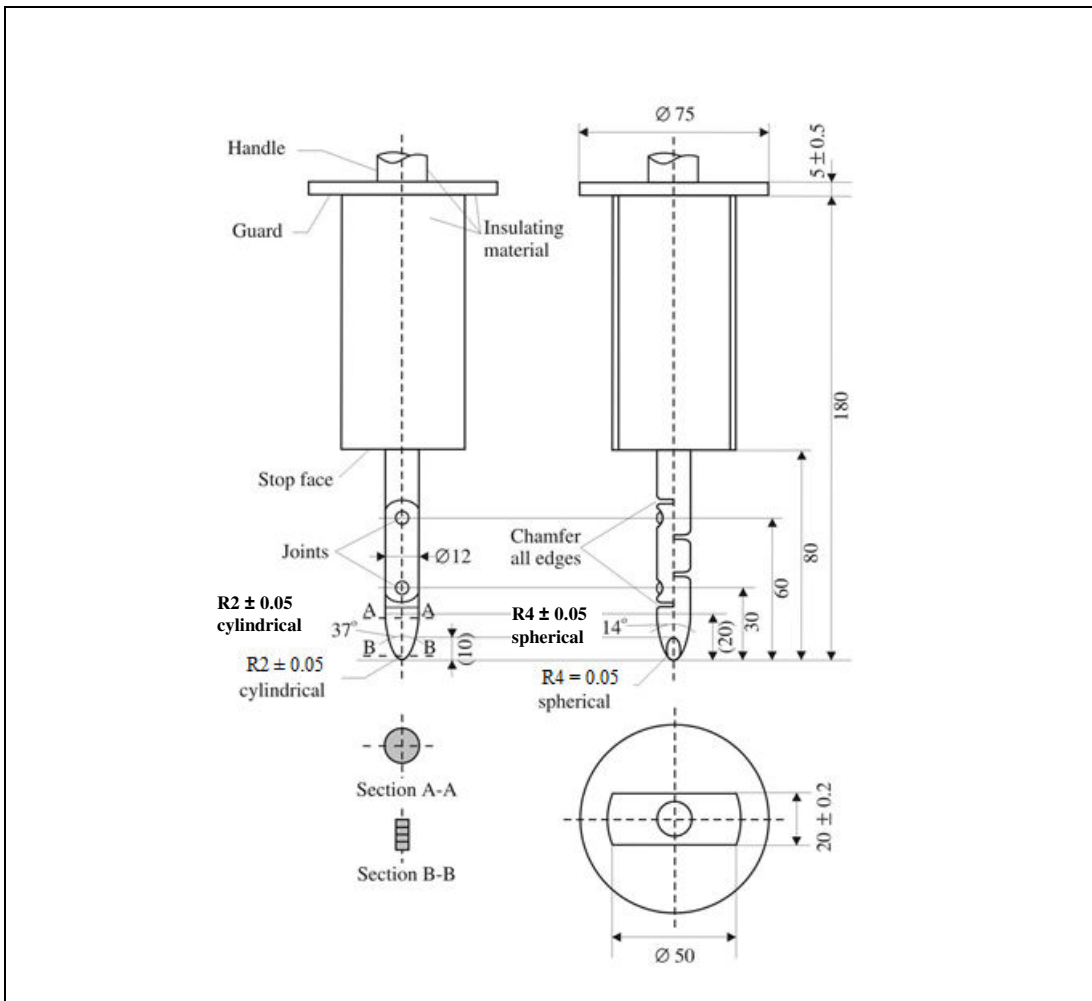
Figure 1 Jointed test finger
