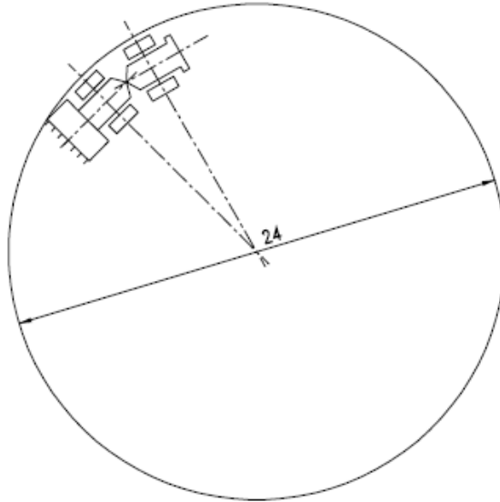
Figure 3 Alternative steering test course
