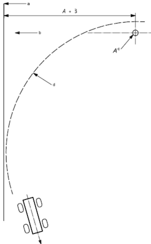
Figure 2 Emergency steering response
