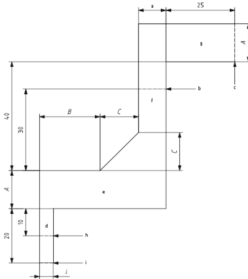
Figure 1 Steering test course
